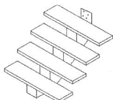
4: Saw Tooth Stringer
